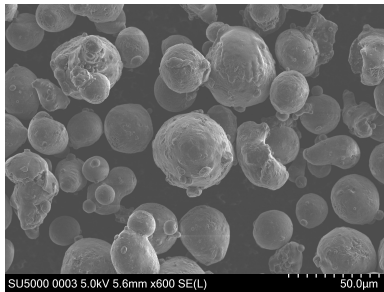
Figure 2: AlSi10Mg powder by IMR. PSD: 20-63 μm. SEM magnification: 600x.
